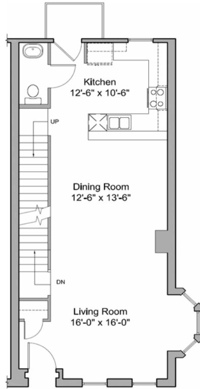
ALTERNATE FIRST FLOOR PLAN
