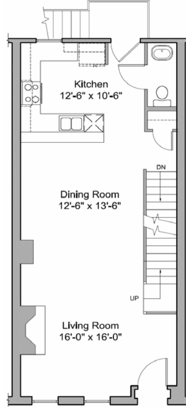
ALTERNATE FIRST FLOOR PLAN
