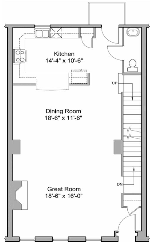
ALTERNATE FIRST FLOOR PLAN
